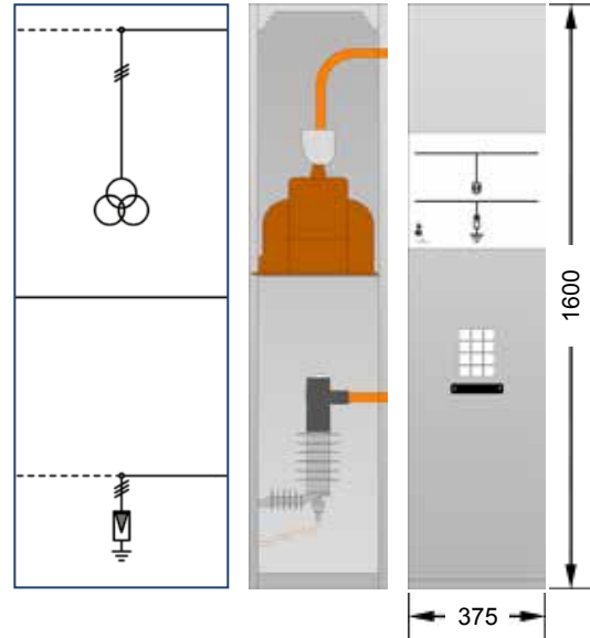
2 VTs Phase-To-Phase only Up to 12kV
