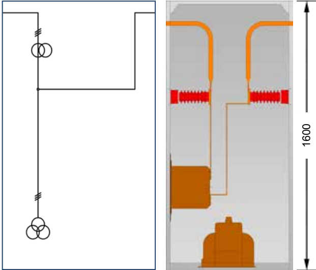
1250A Available Version
