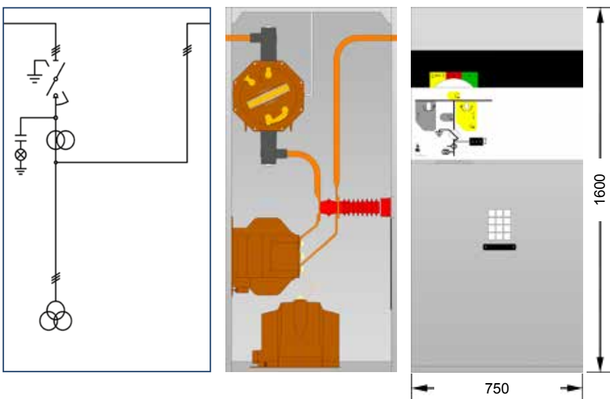
Max 2 VTs Phase-To-Phase + 3 VTs Phase-To-Earth
