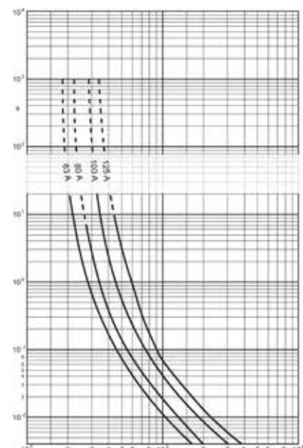
Special fuses up to 24kV
