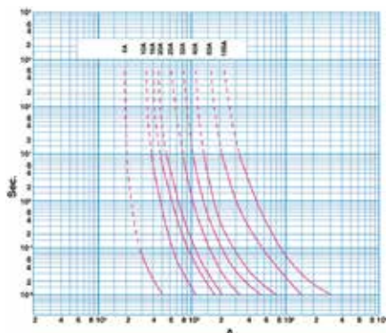
Standard fuses
