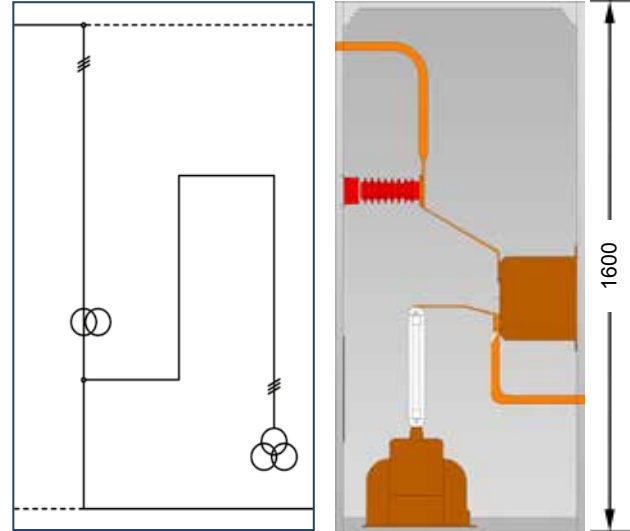
1250A Available Version
