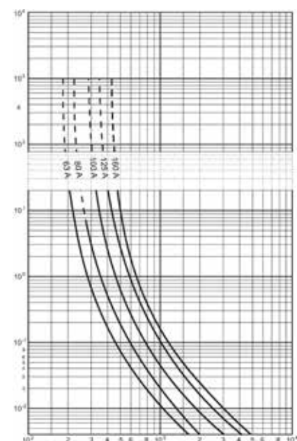
Special fuses up to 12kV
