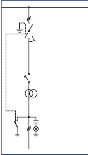
1250A Available Version
